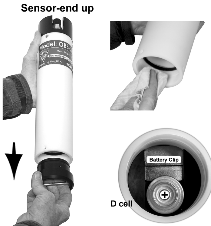
FIGURE 6-2. Battery installation
