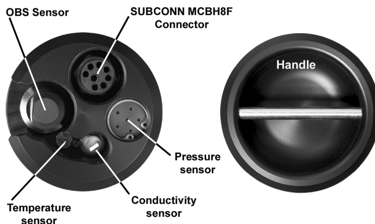
FIGURE 6-1. Components
